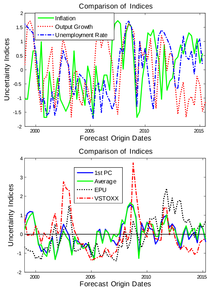
Figure 3. Comparing Uncertainty Indices
