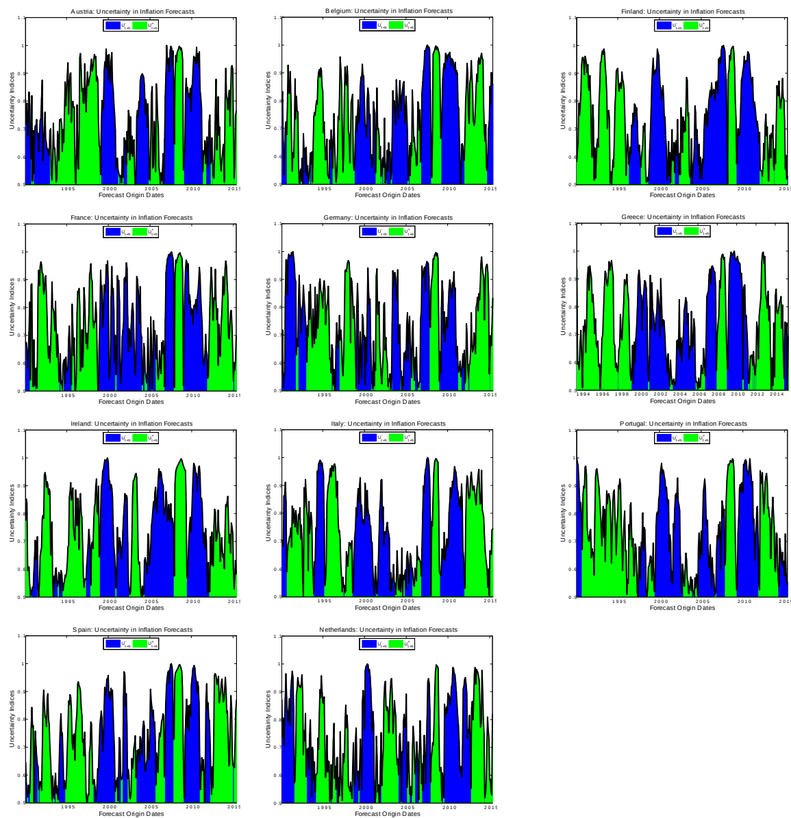
Figure 8. Euro Area Country-Specific Monthly Inflation Uncertainty Indices
