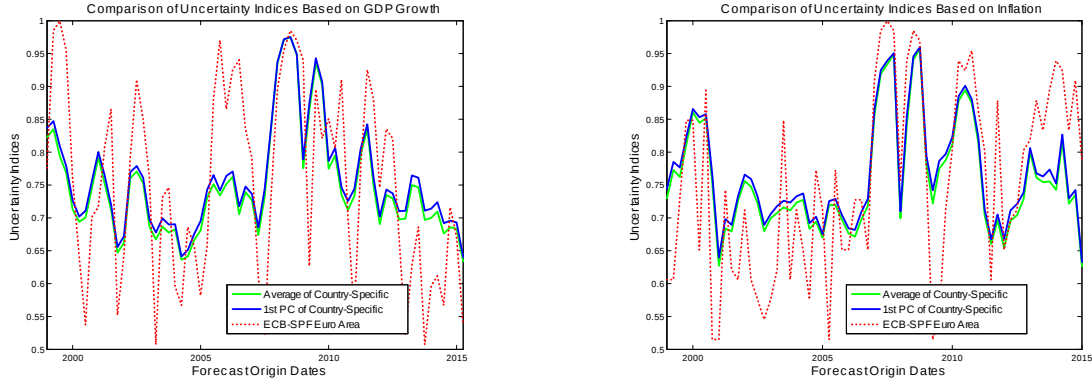
Figure 6. ECB-SPF Euro Area vs. the Aggregate of Country-Specific Indices
