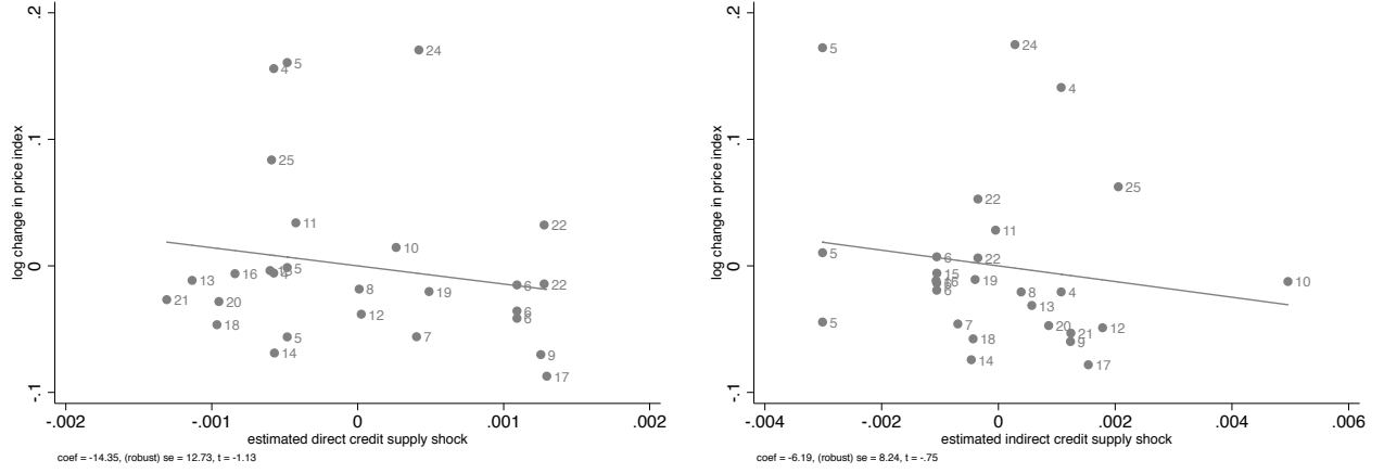
Figure 6: Change in industrial price indexes and credit supply shocks
