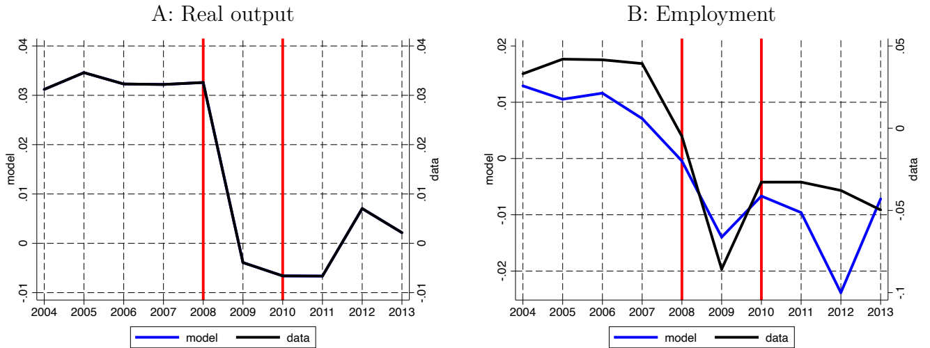
Figure 9: Evolution of employment and output: model vs. data
