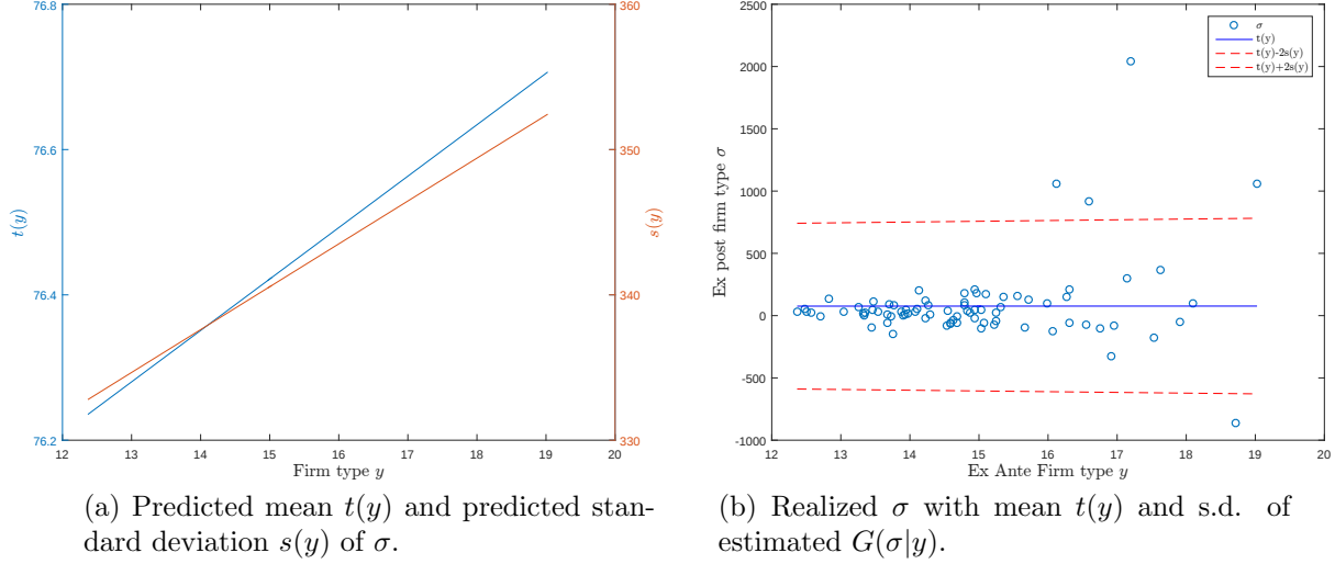
Figure 4: Estimated Parameters t, s .
