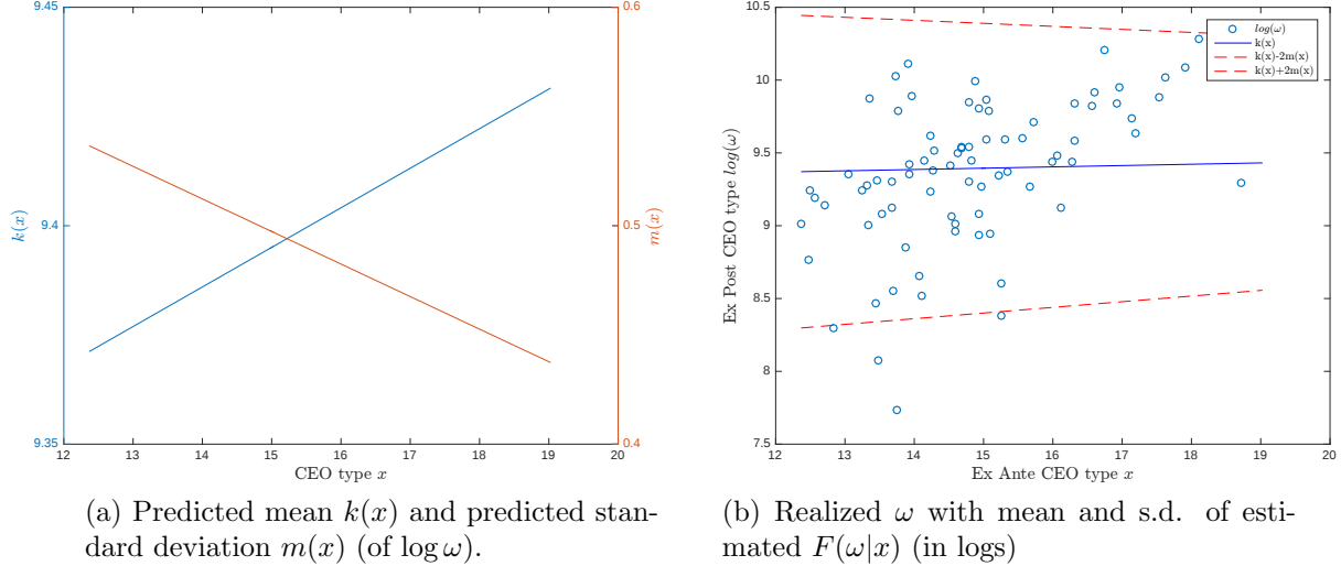
Figure 3: Estimated Parameters k, m .
