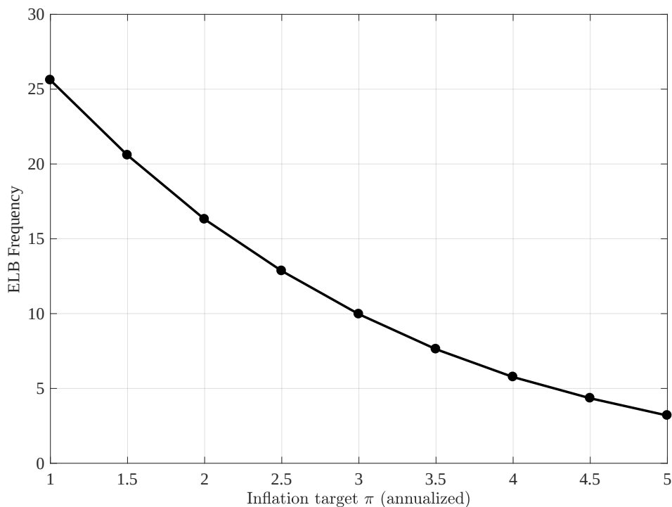
Figure A.1: Probability of ELB
