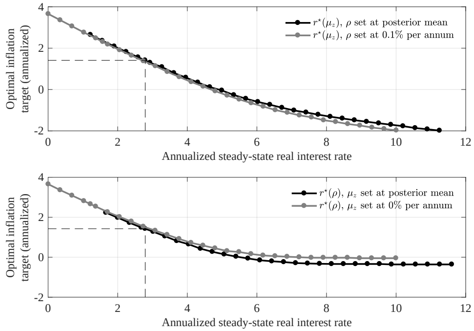
Figure B.1: (r^*, \pi^*) relation with near-zero r^*
