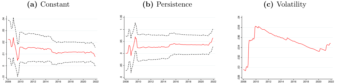
Figure B.8 – Rolling Estimates for Inflation Parameters
