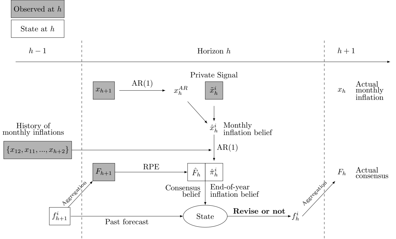
Figure VII – Model Timeline
