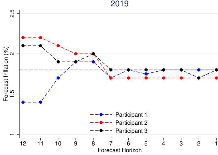
Figure II – Fixed-event forecasting
