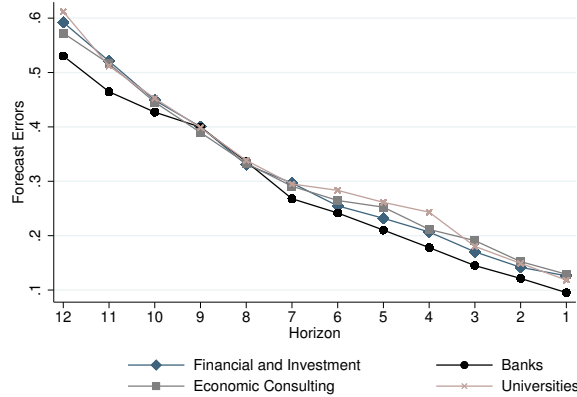
Figure A.7 – Forecast Errors by Groups
