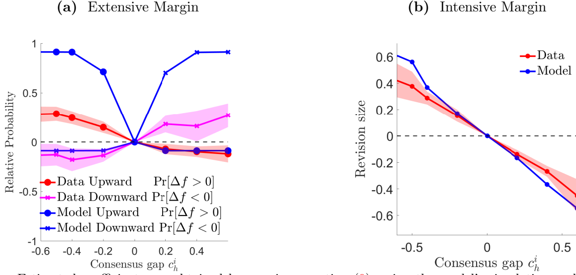
Figure XIII – Untargetted Extensive and Intensive Margins
