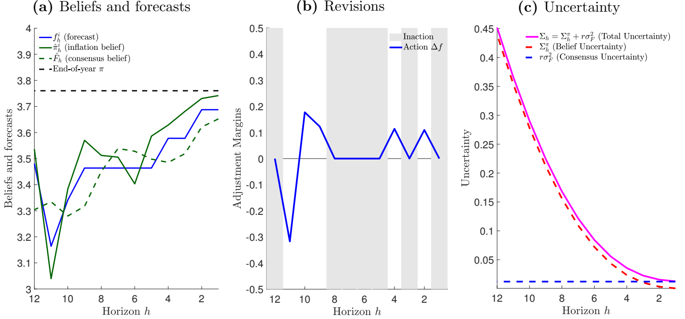
Figure IX – Forecaster-level dynamics
