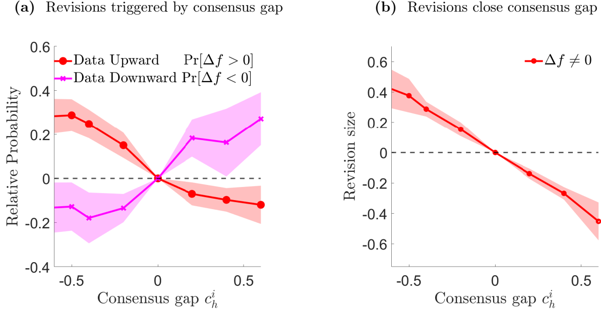
Figure V – Consensus Triggers Revisions
