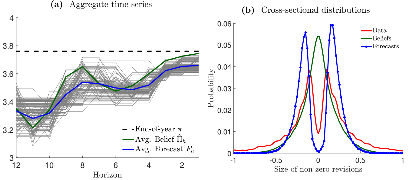
Figure X – Aggregate dynamics
