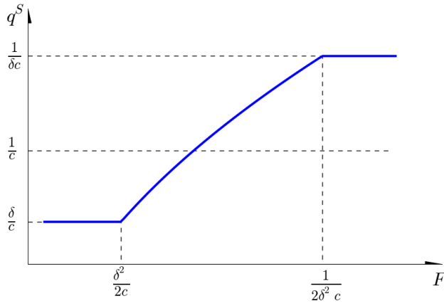
Figure 1: Quality provision in the symmetric equilibrium (quadratic cost).
